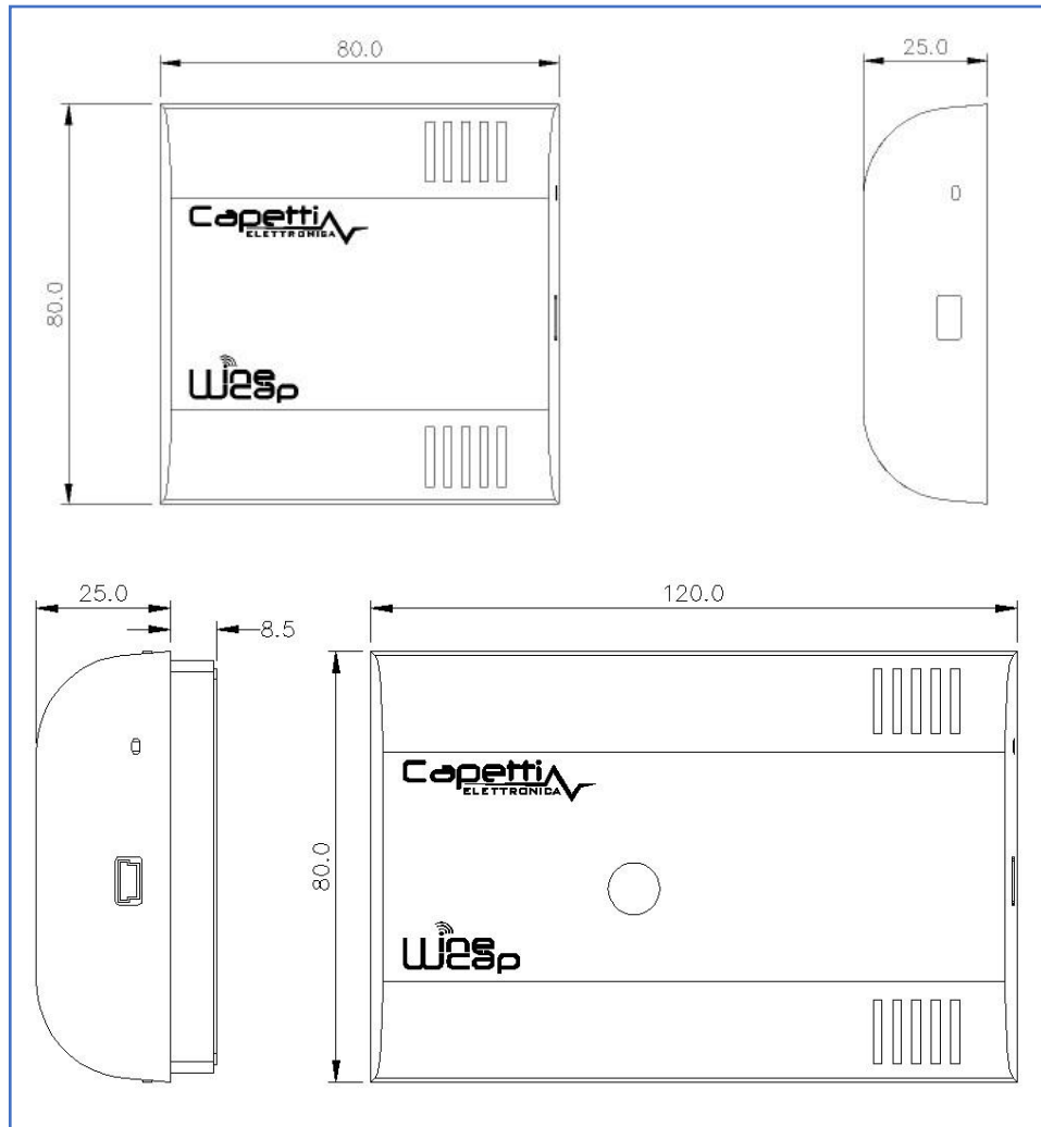
Picture 7 - Mechanical dimensions
