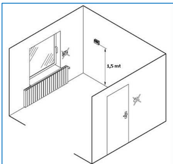
Picture 1 - Sensor positioning
