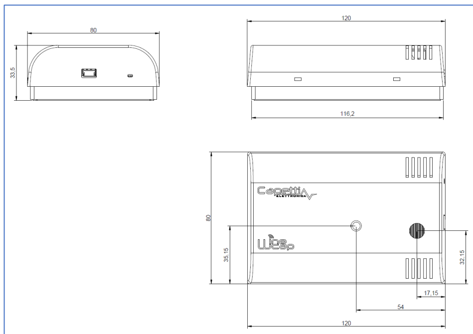
Picture 6 - Mechanical dimensions
