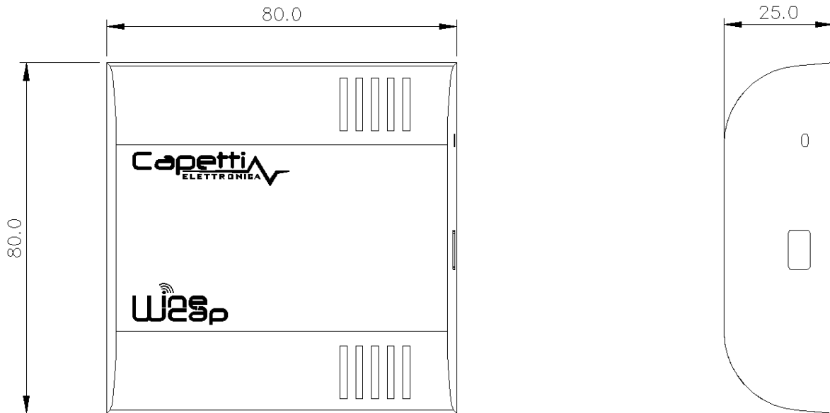
Picture 8 - Mechanical dimensions
