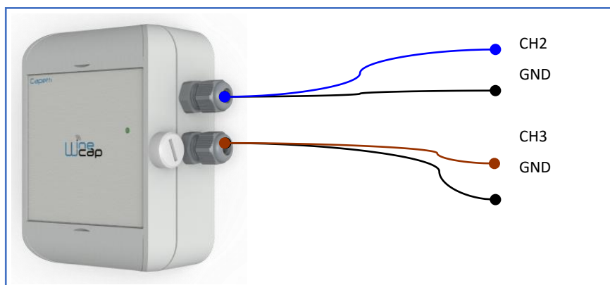
Picture 7 - Connections layout
