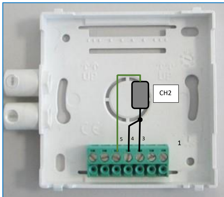
Picture 7 - Connections layout
