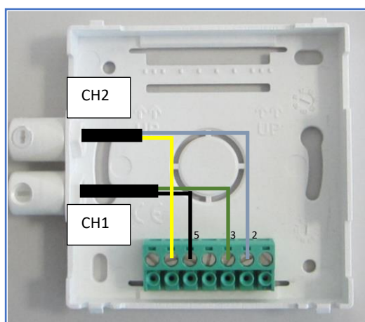
Picture 7 - Connections layout
