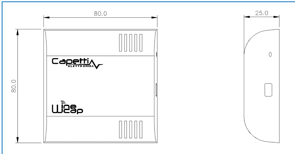
Picture 8 - Mechanical dimensions
