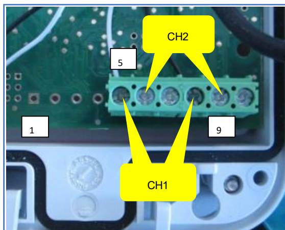
Picture 7 - Connections layout
