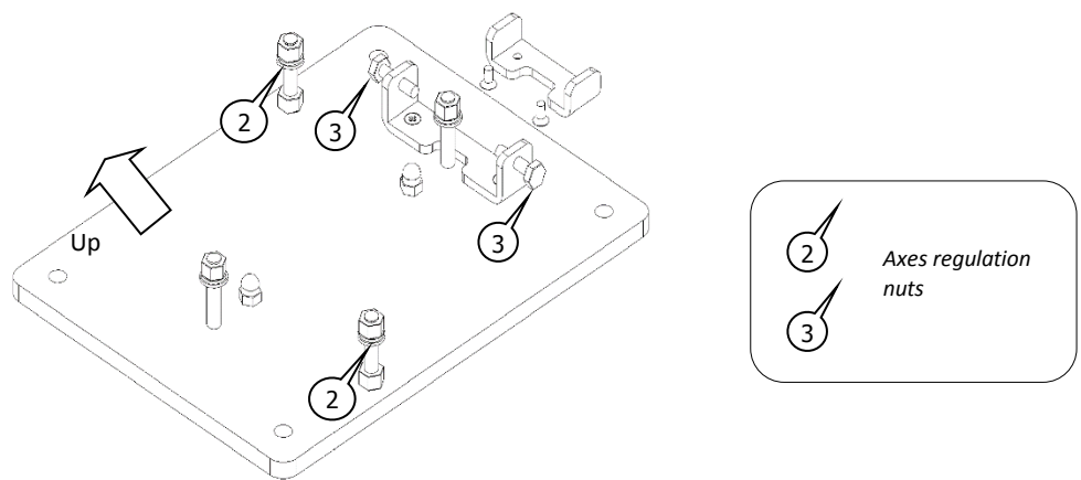
Picture 3 - FIX-WSD15 Micrometric regulation slab
