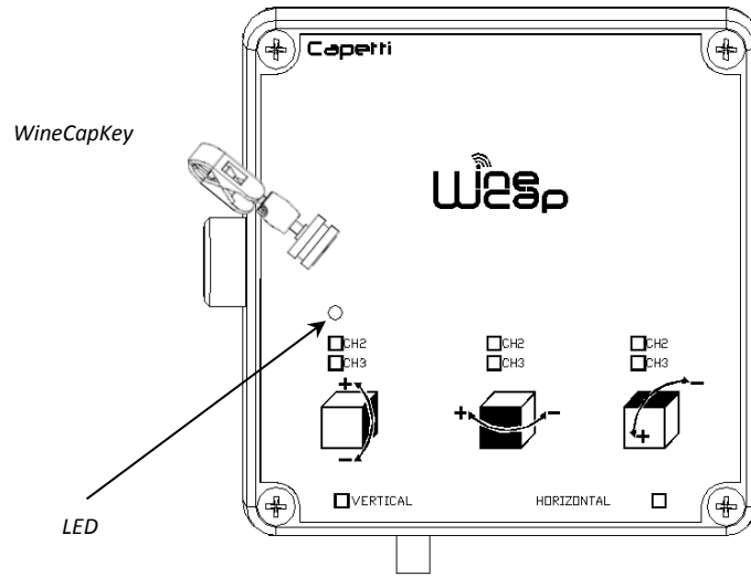
Picture 7 - WineCapKey positioning
