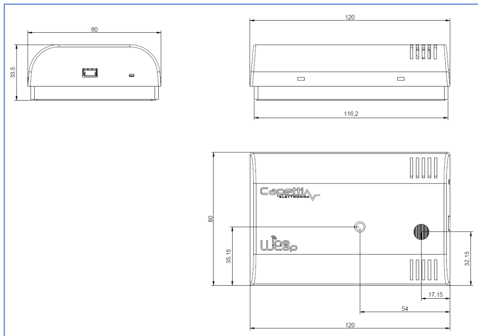
Picture 7 - Mechanical dimensions
