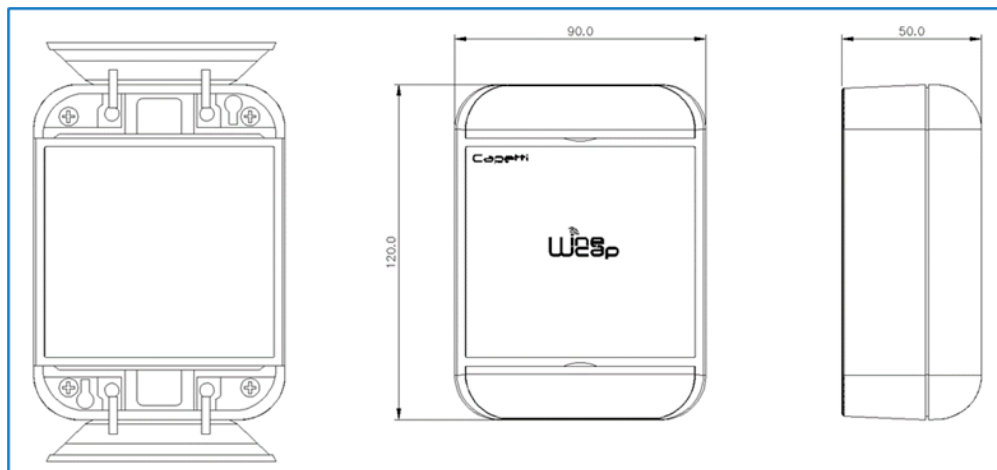
Picture 8 - Mechanical dimensions
