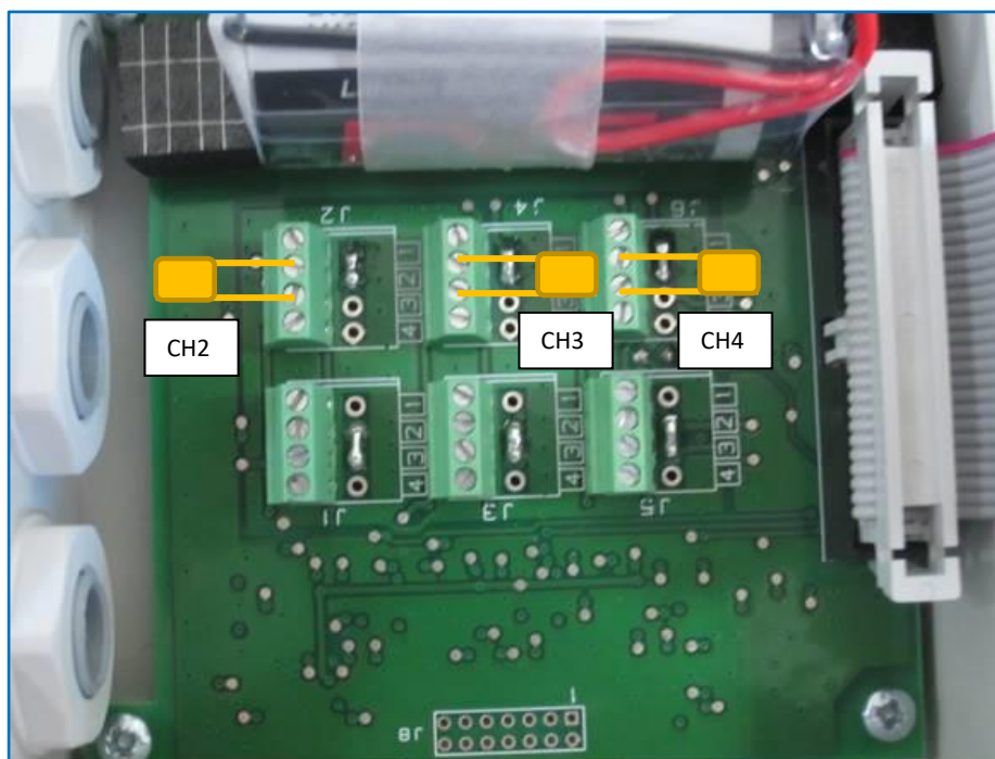
Picture 7 - Connections layout
