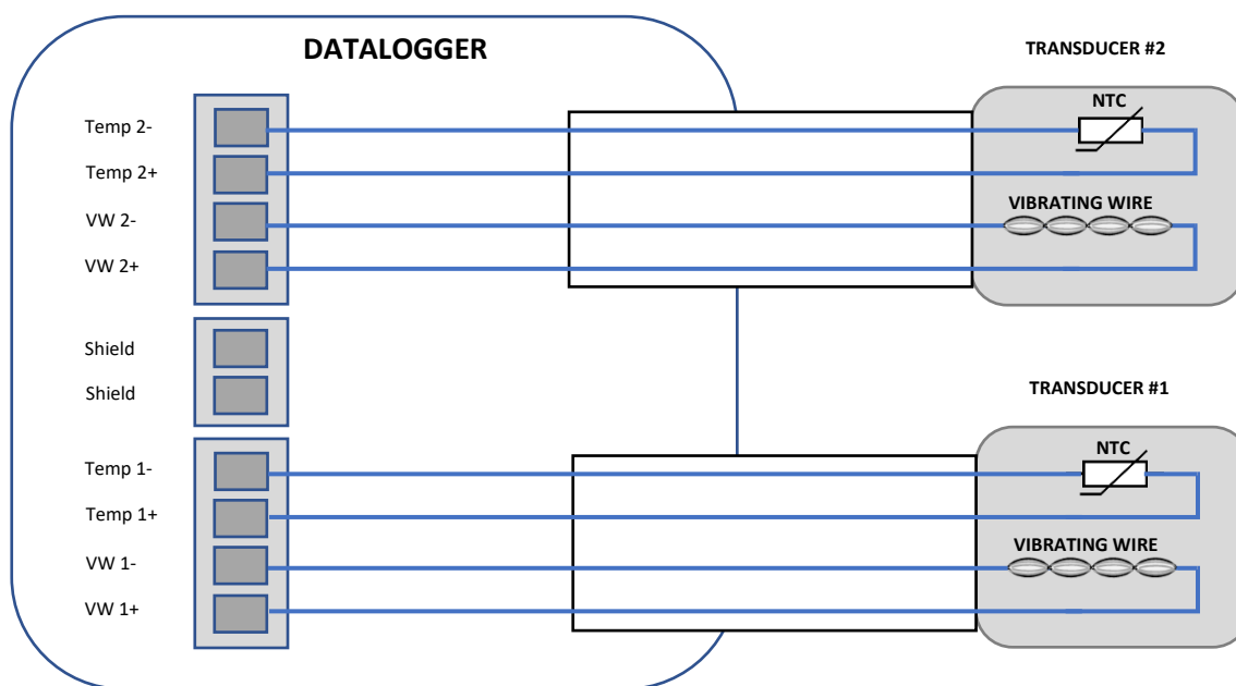
Picture 6 - Connections layout
